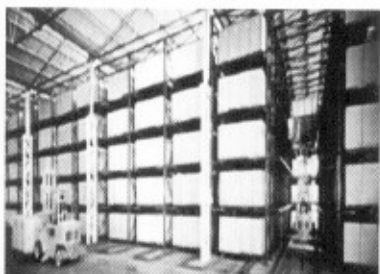
Drive-in Racking
